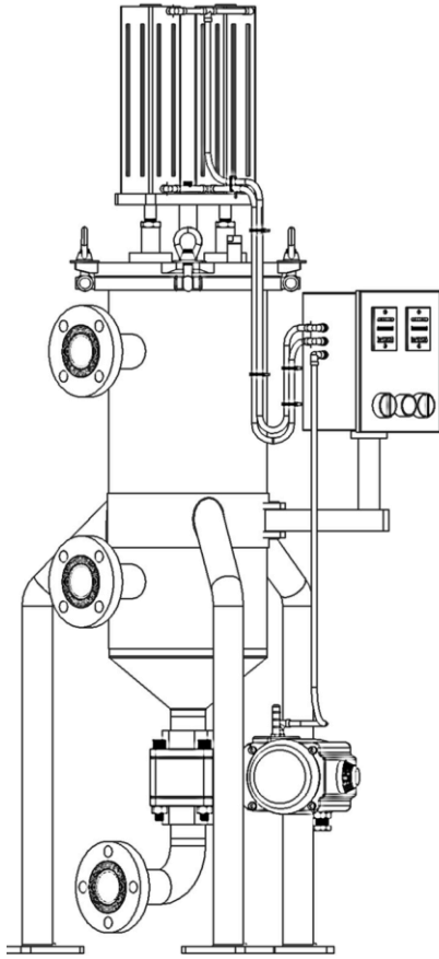
With Logical Pneumatic Controller
