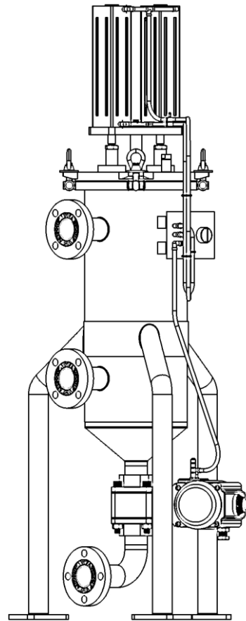
With Logical Electric Controller
